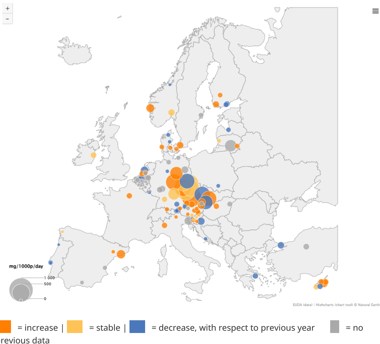
Figure 10. Changes in the mean weekly methamphetamine metabolites from wastewater analyses in selected European cities between 2024 and 2025
