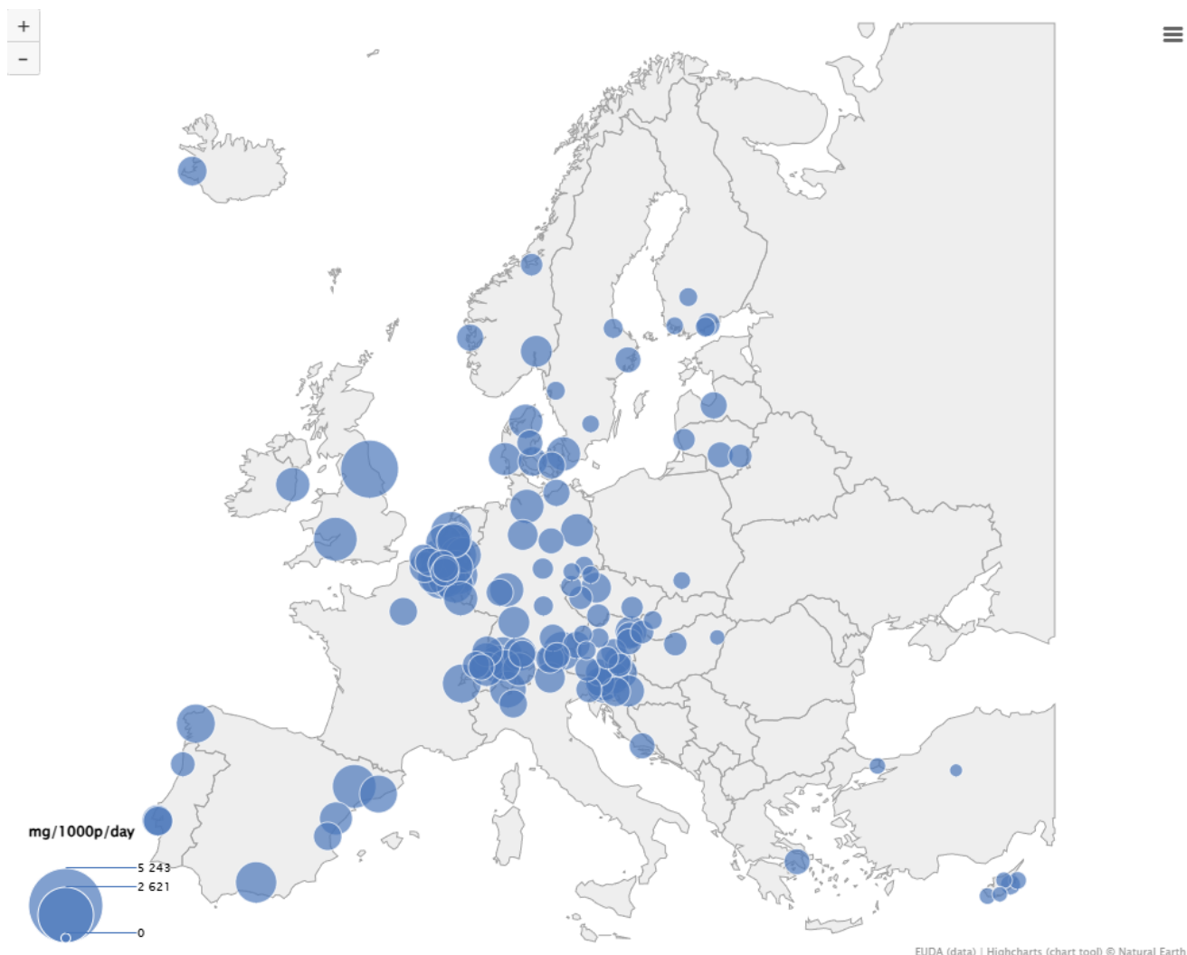
Figure 3. Relative geographical distribution of cocaine metabolite as detected in European cities, 2025 (daily mean)
