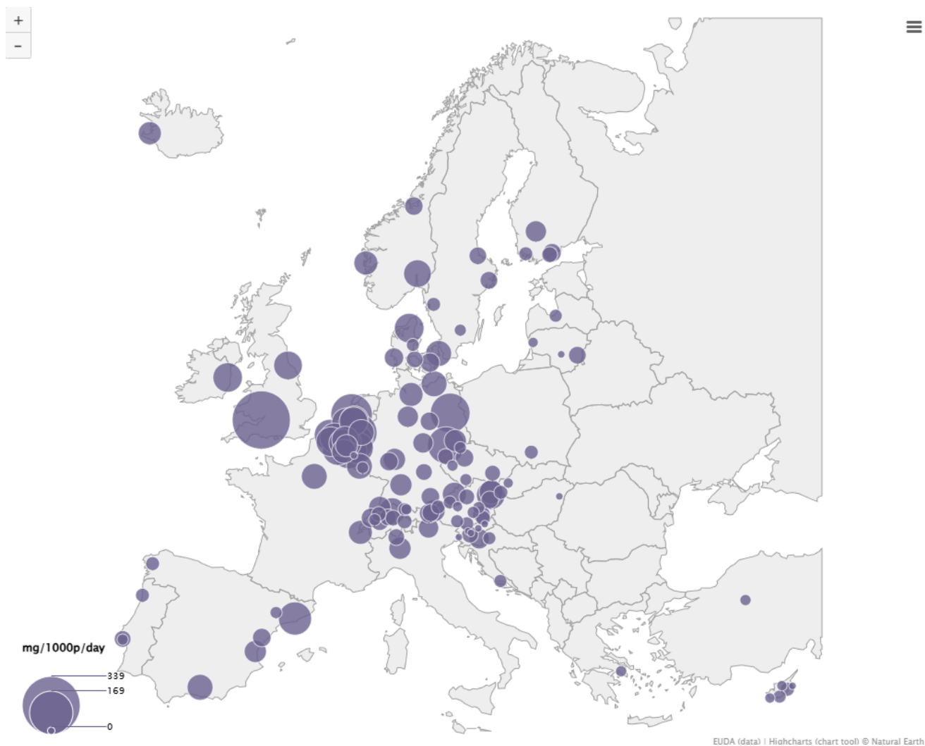
Figure 11. Relative geographical distribution of ketamine residues as detected in European cities, 2025 (daily mean)
