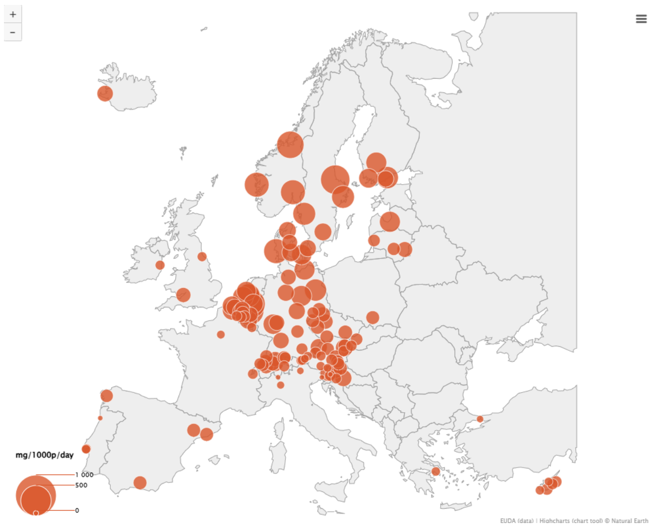
Figure 7. Relative geographical distribution of amphetamine residues as detected in European cities, 2025 (daily mean)
