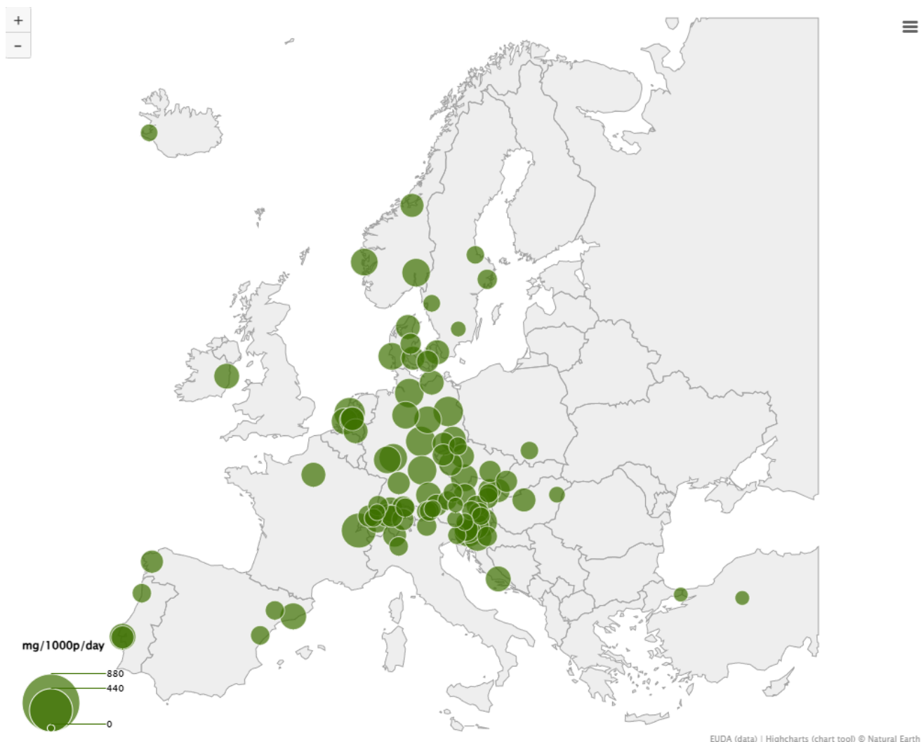
Figure 1. Relative geographical distribution of cannabis metabolite as detected in European cities, 2025 (daily mean)
