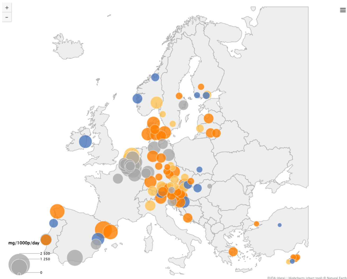
Figure 4. Changes in the mean weekly cocaine metabolites from wastewater analyses in selected European cities between 2024 and 2025
