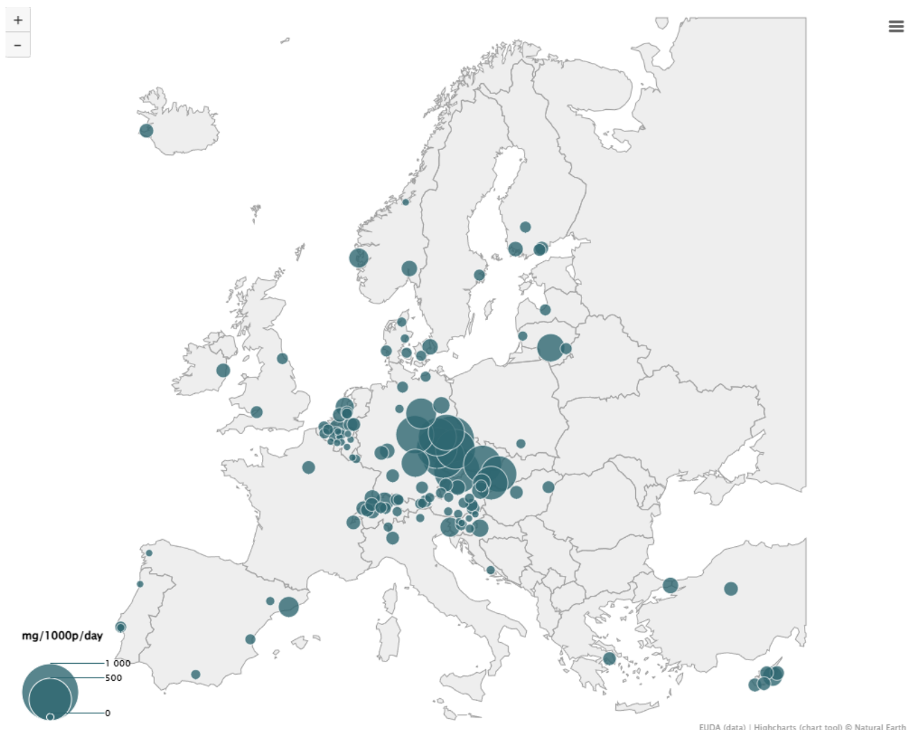
Figure 9. Relative geographical distribution of methamphetamine residues as detected in European cities, 2025 (daily mean)
