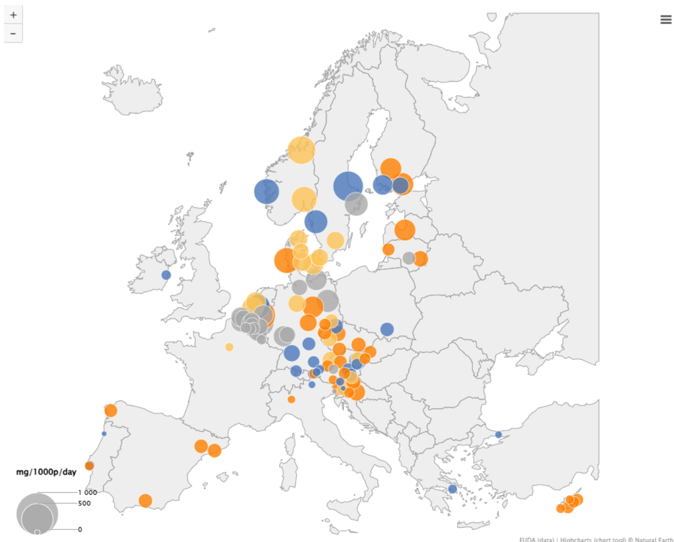
Figure 8. Changes in the mean weekly amphetamine metabolites from wastewater analyses in selected European cities between 2024 and 2025
