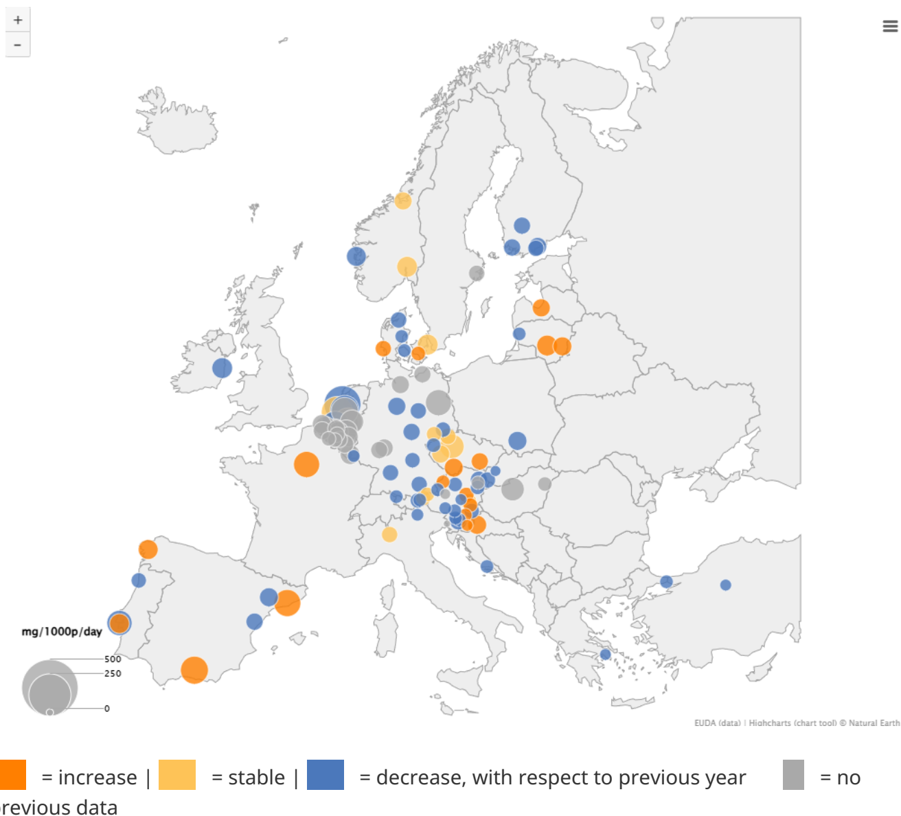
Figure 6. Changes in the mean weekly MDMA metabolites from wastewater analyses in selected European cities between 2024 and 2025
