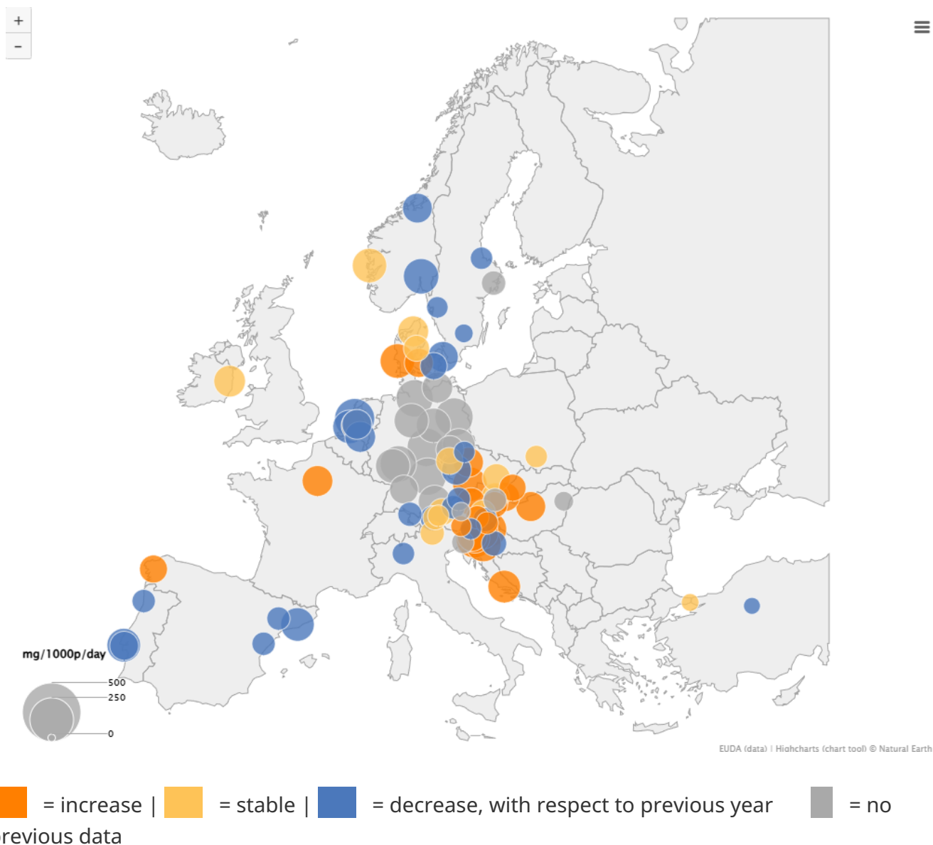
Figure 2. Changes in the mean weekly cannabis metabolites from wastewater analyses in selected European cities between 2024 and 2025
