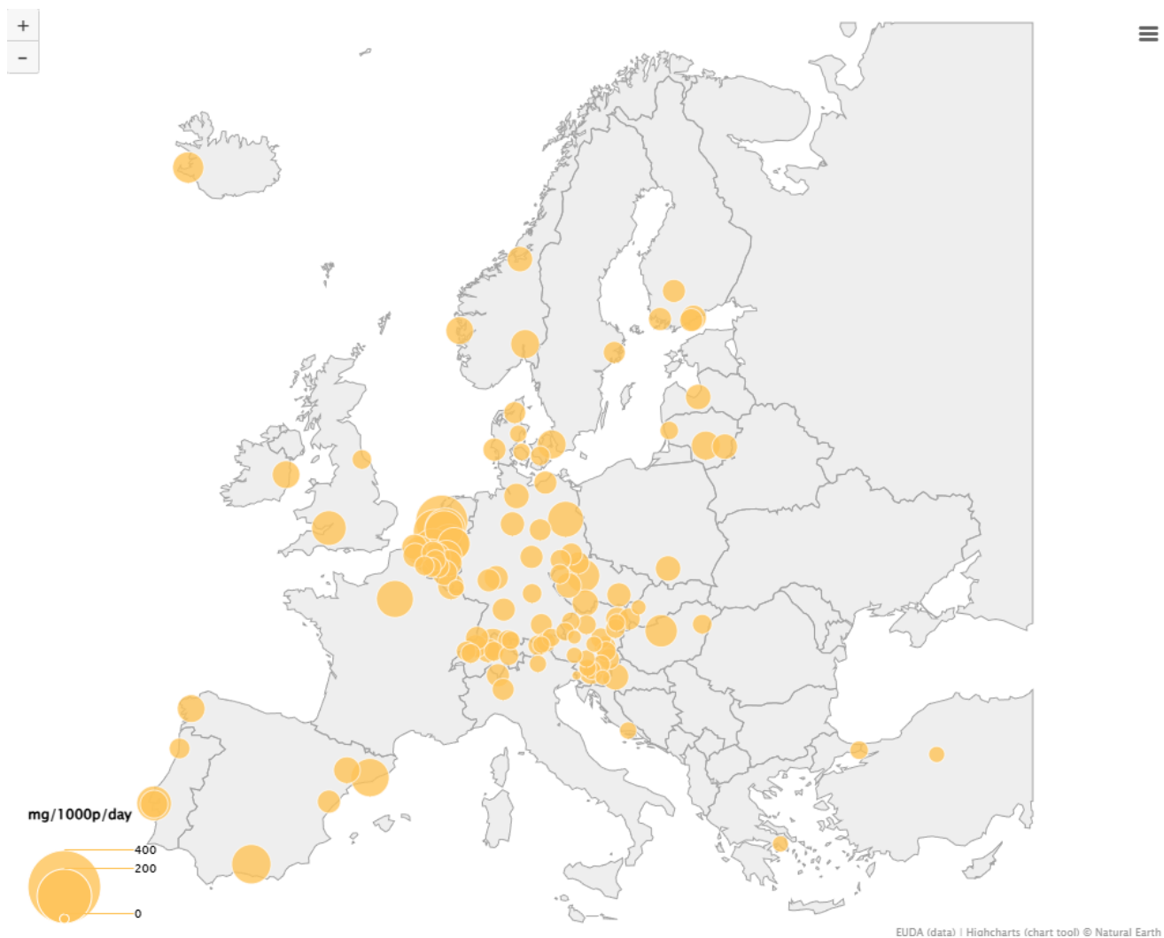
Figure 5. Relative geographical distribution of MDMA residues as detected in European cities, 2025 (daily mean)
