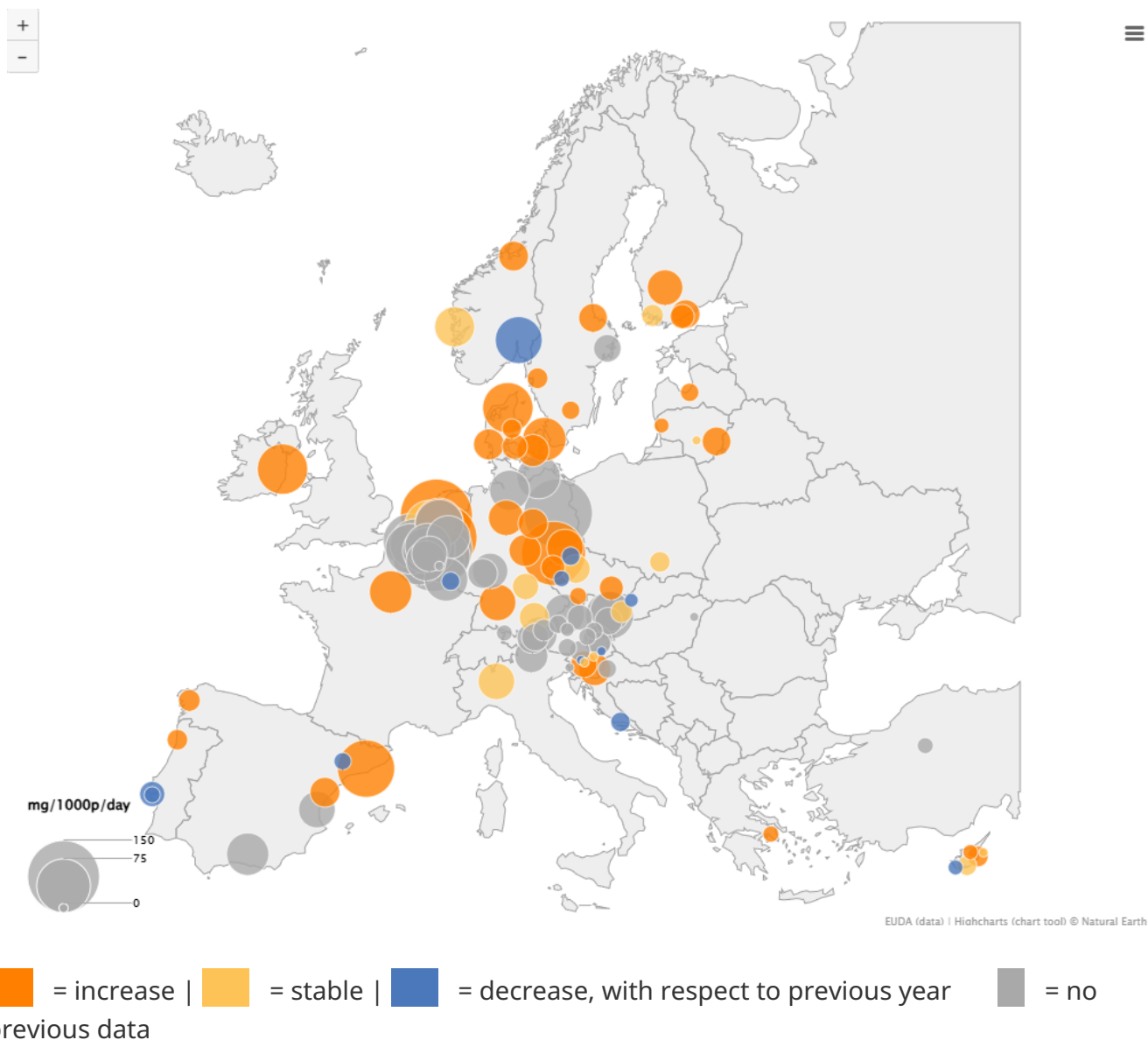
Figure 12. Changes in the mean weekly ketamine metabolites from wastewater analyses in selected European cities between 2024 and 2025
